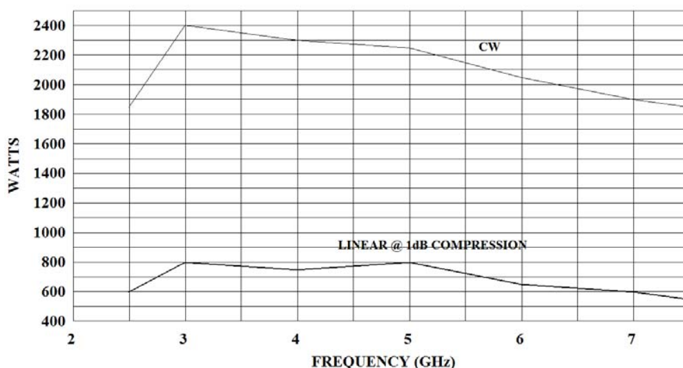
1500T2G8A TYPICAL POWER OUTPUT
