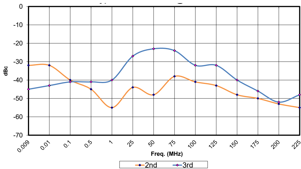
TYPICAL HARMONICS @ 7500 WATTS
