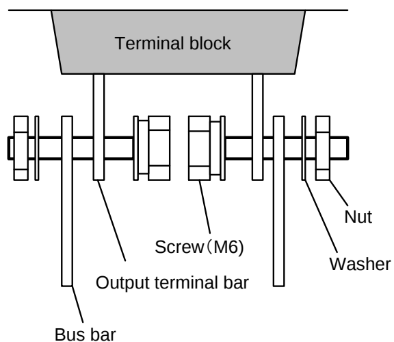
Parallel connection kit for vertical installation PSB-004
