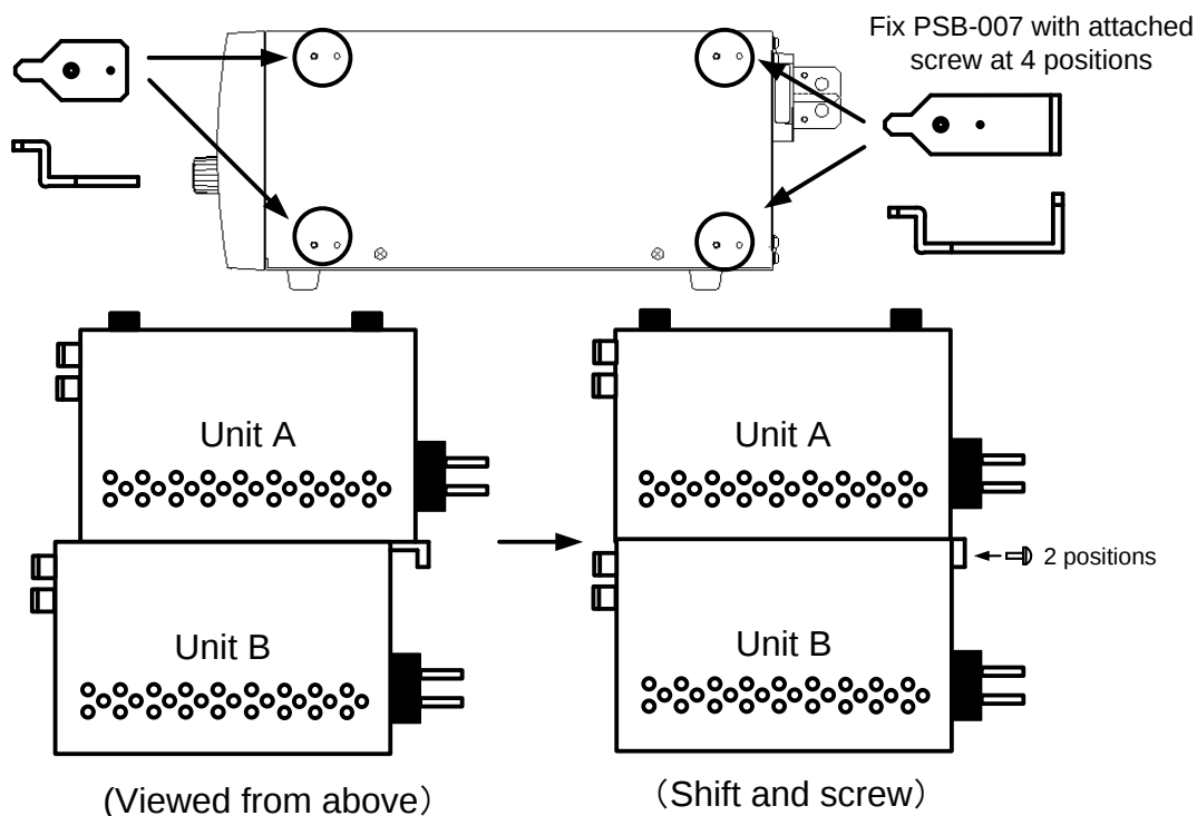
Connection for Horizontal Installation
