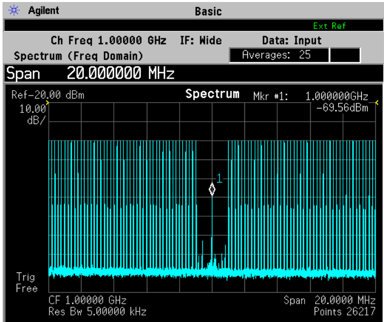
Figure 2-6 Spectrum Measurement - Spectrum View with Opt. 122–80 MHz Bandwidth Digitizer Hardware
