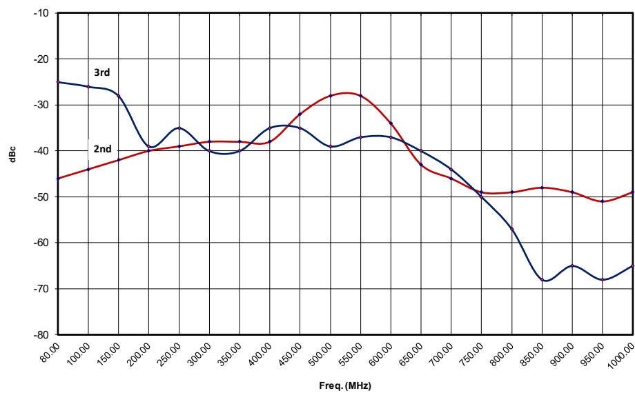
TYPICAL HARMONICS @ 100 WATTS
