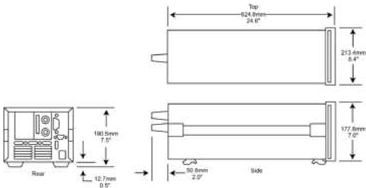
Keysight N3301A
