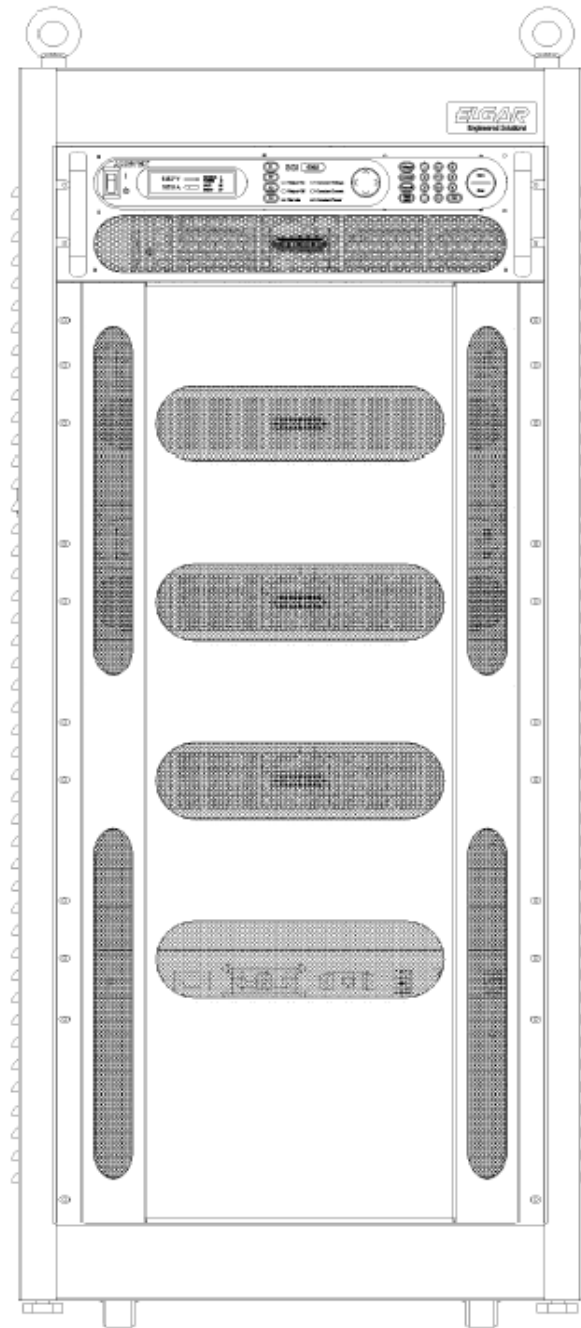
Figure 2-5 - 24U HPX Power Rack, Front View
