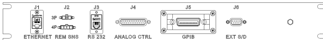
Figure 2-4 - HPX I/O Panel
