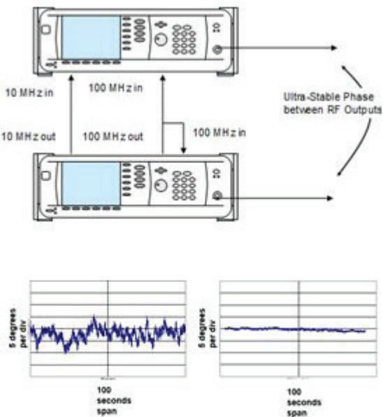
Figure 4. Precision Clock Source Setup
