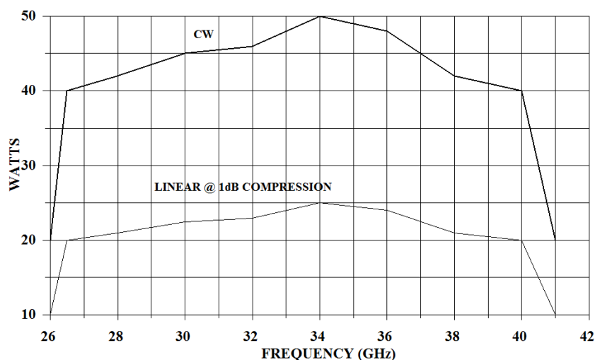
40T26G40A TYPICAL POWER OUTPUT
