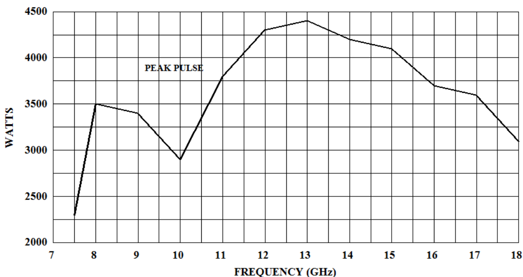
2000TP8G18 TYPICAL POWER OUTPUT
