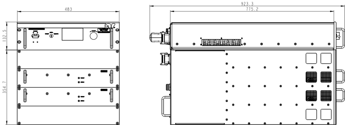
Units=mm; base model 5000SP2G4 shown
