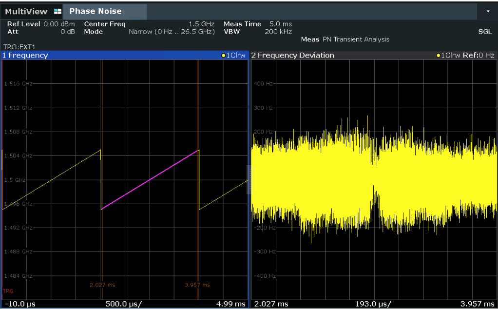
Analysis of FMCW chirp linearity. Left: the pink reference line can be seen. Right: the deviation of the frequency from linear behavior is displayed.
