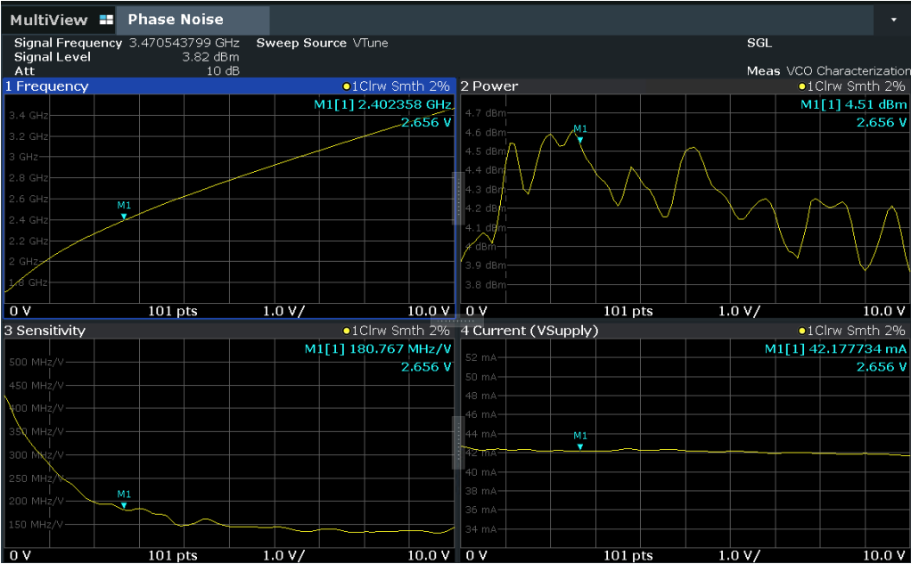
A typical VCO measurement. Key parameters such as frequency, power, sensitivity and current consumption are measured relative to the tuning voltage.
