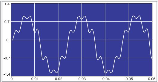
Harmonic Waveform
