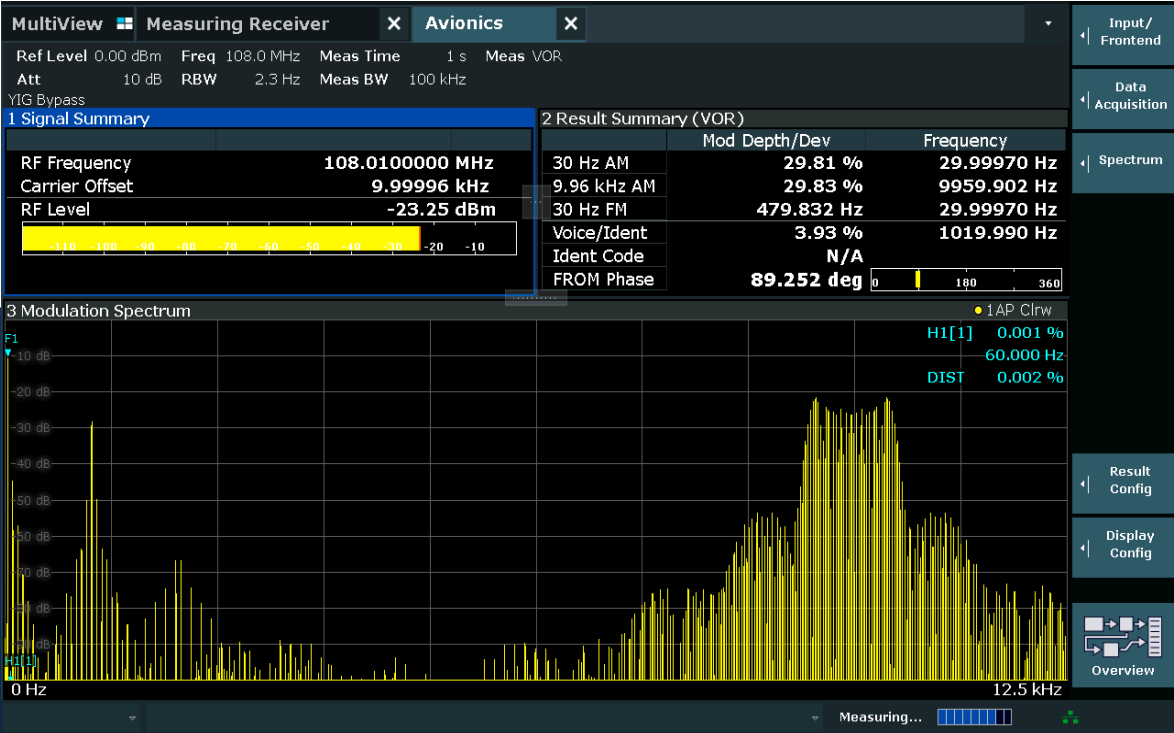
Analysis of a VOR signal: The spectrum, power and modulation parameters are displayed.
