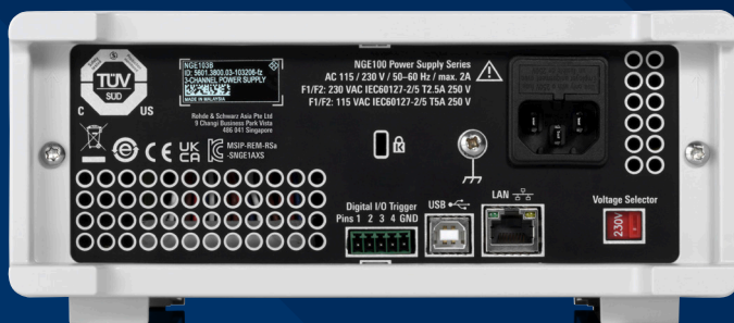
Rear view of the R&S®NGE103B
