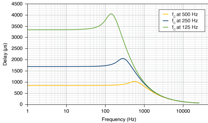
Figure 1. Butterworth Filter Input Delay (2nd Order, with 12.8 MHz Timebase, 4000 Hz, 2000 Hz, 1000 Hz)
