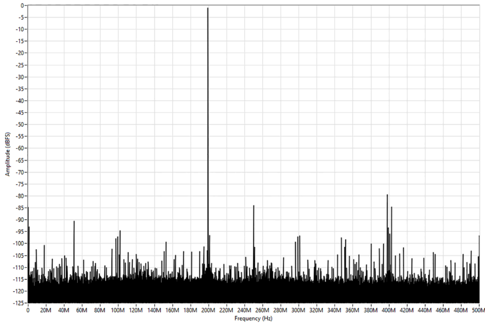
Figure 3. AC-Coupled Single Tone Spectrum (199.1 MHz, -1 dBFS, 1 kHz RBW), Measured
