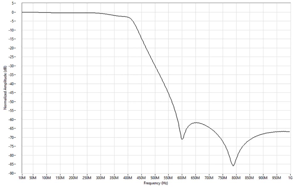
Figure 10. DC-Coupled Frequency Response Zoomed In, Measured
