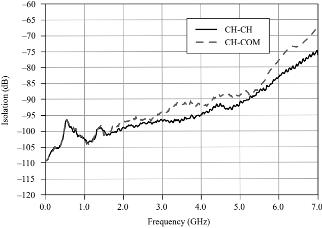
Figure 3. Typical Isolation
