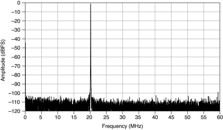
Figure 2. Analog Input One-Tone Spectral Measurement (20.17 MHz, -1 dBFS)
