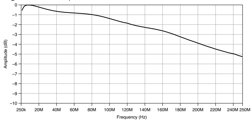
Figure 1. AC-Coupled Passband
