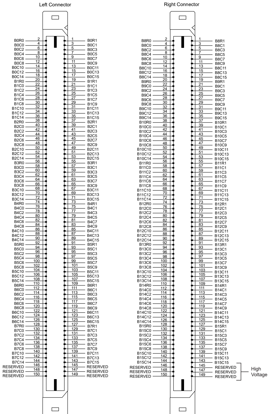
Figure 1. PXI-2532B Pinout
