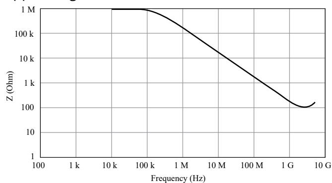
Figure 2. SA2500X Typical Input Impedance. Input impedance decreases as the frequency of the applied signal increases.
