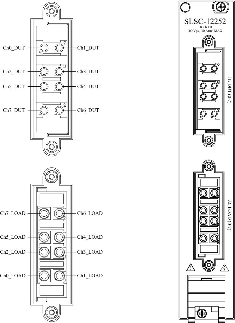
Figure 1. SLSC-12252 Pinout
