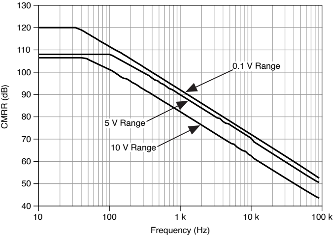
Figure 1. AI <0..31> CMRR
