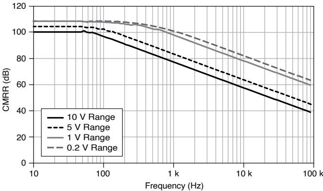
Figure 3. AI CMRR
