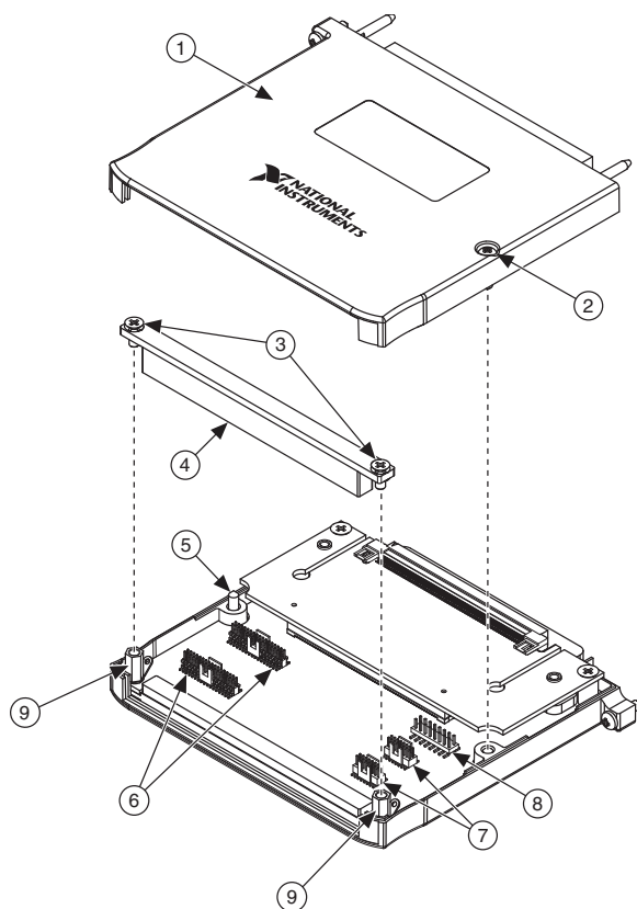
Figure 1. NI TB-2641B Terminal Block
