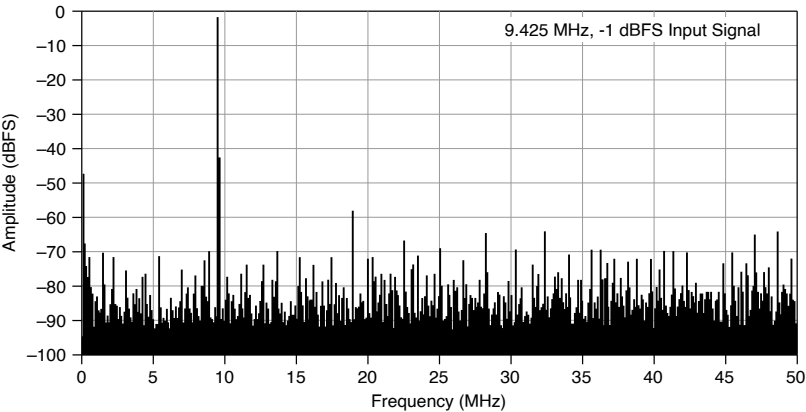
Figure 2. USB-5133 Dynamic Performance, 1 V pk-pk Range, 524,288-Point FFT, Measured
