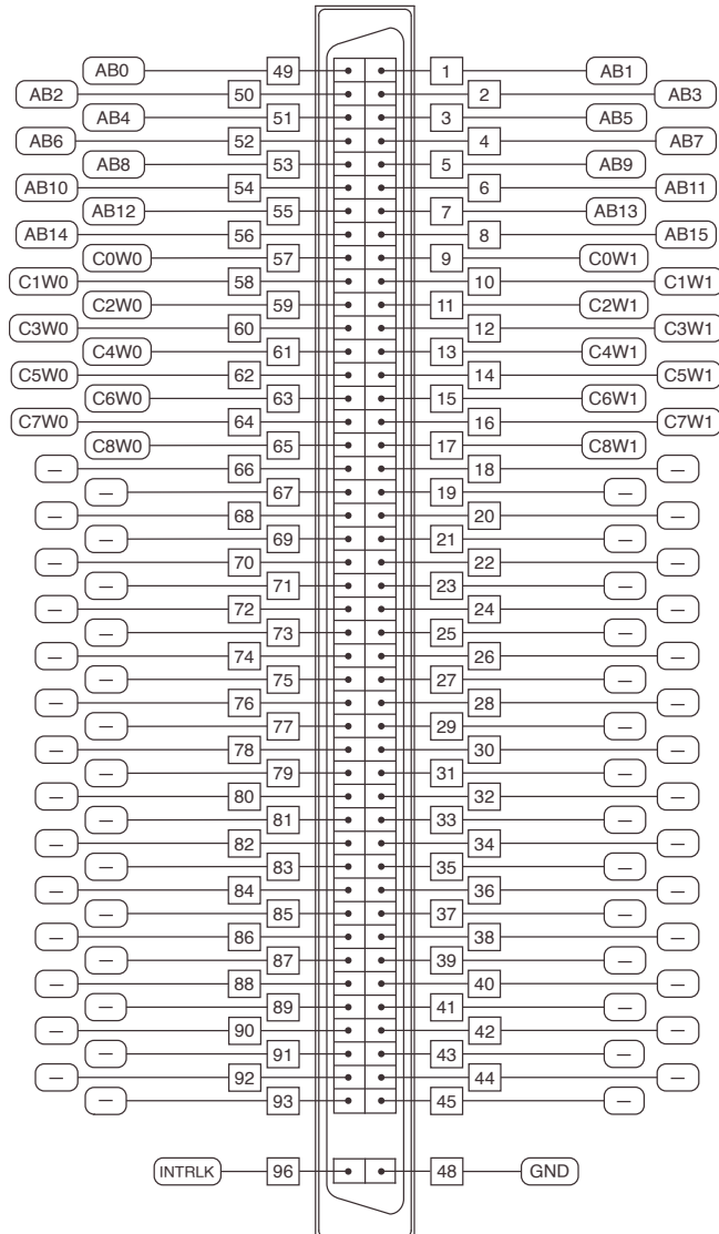
Figure 1. NI 2814A/B Connector Pinout
