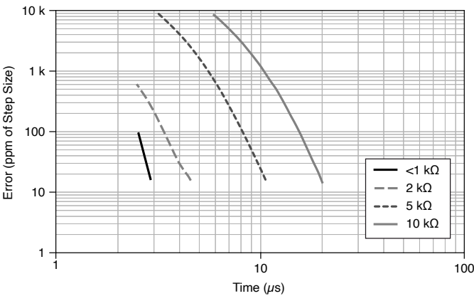
Figure 3. Settling Error versus Time for Different Source Impedances
