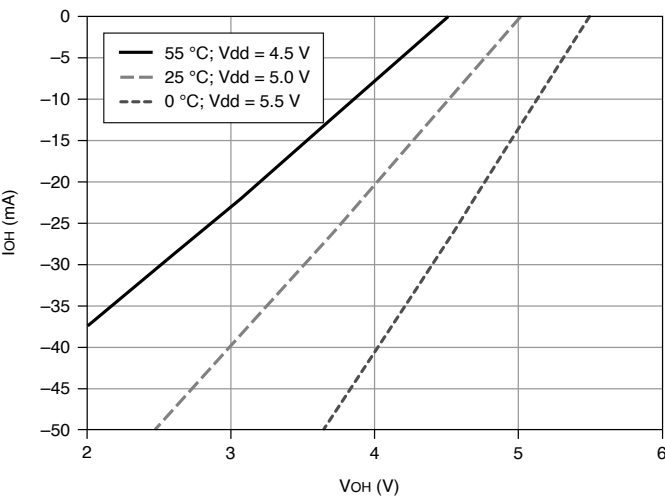
Figure 3. PFI <0..15>/P0.<0..15>: I_{OH} versus V_{OH}
