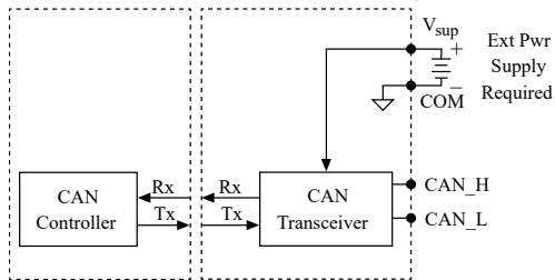
Figure 3. NI-9882 Block Diagram
