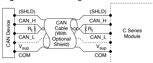
Figure 1. Connecting the NI-9882 to a CAN Device
