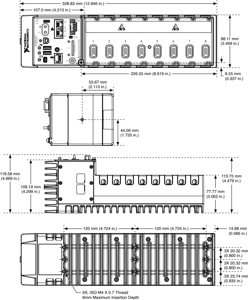
Figure 1. cDAQ-9133 Dimensions
