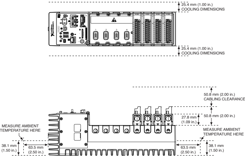
Figure 1. cDAQ-9133 Temperature, Cooling, and Cabling Dimensions
