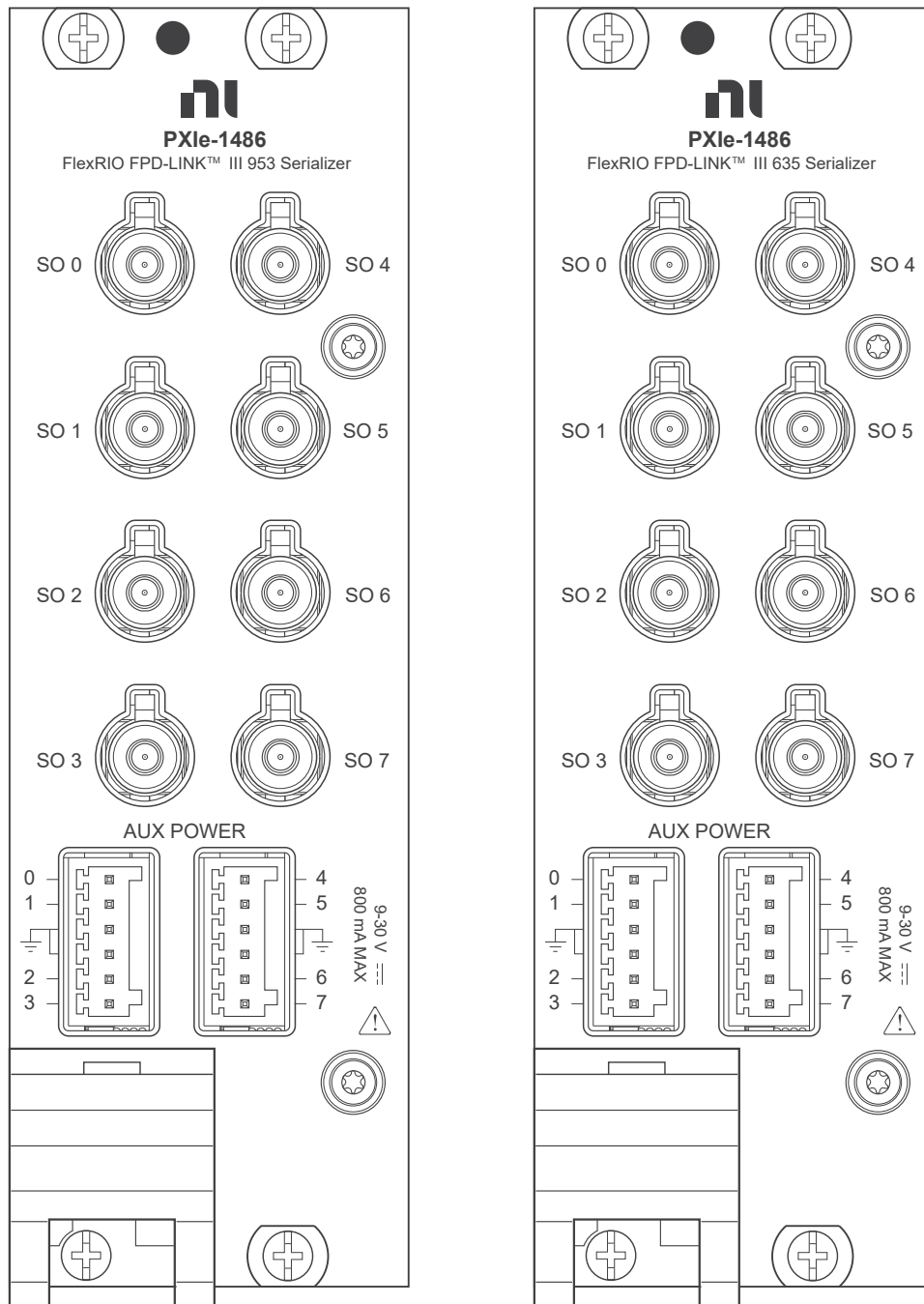
Figure 8. Serializer Front Panels
