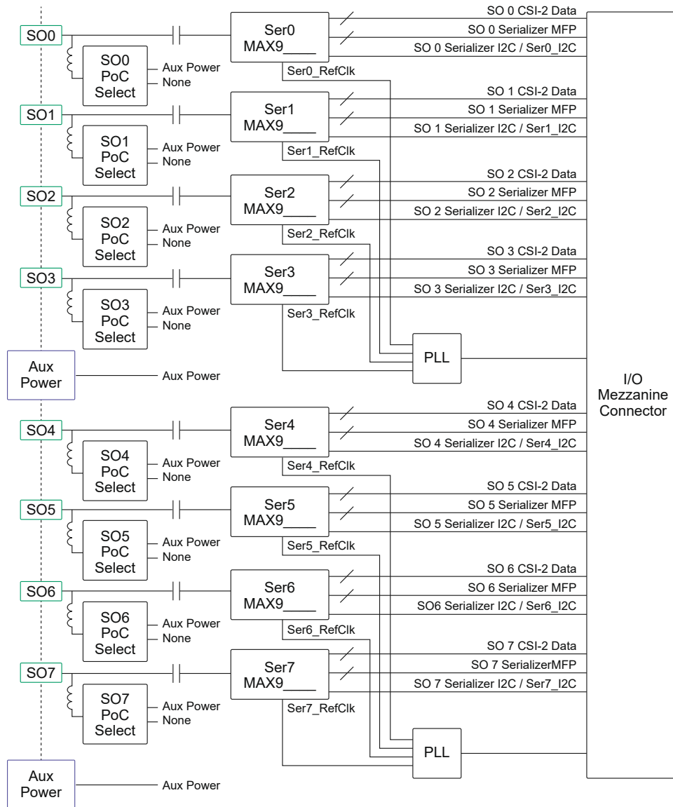
Figure 13. Serializer Block Diagram
