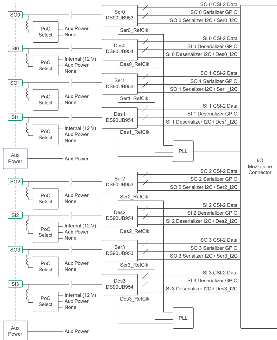
Figure 14. SerDes Block Diagram
