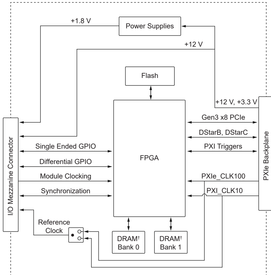
Figure 15. PXIe-1486 FPGA Block Diagram
