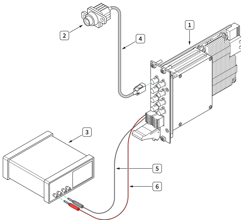
Figure 3. PXle-1486 Deserializer
