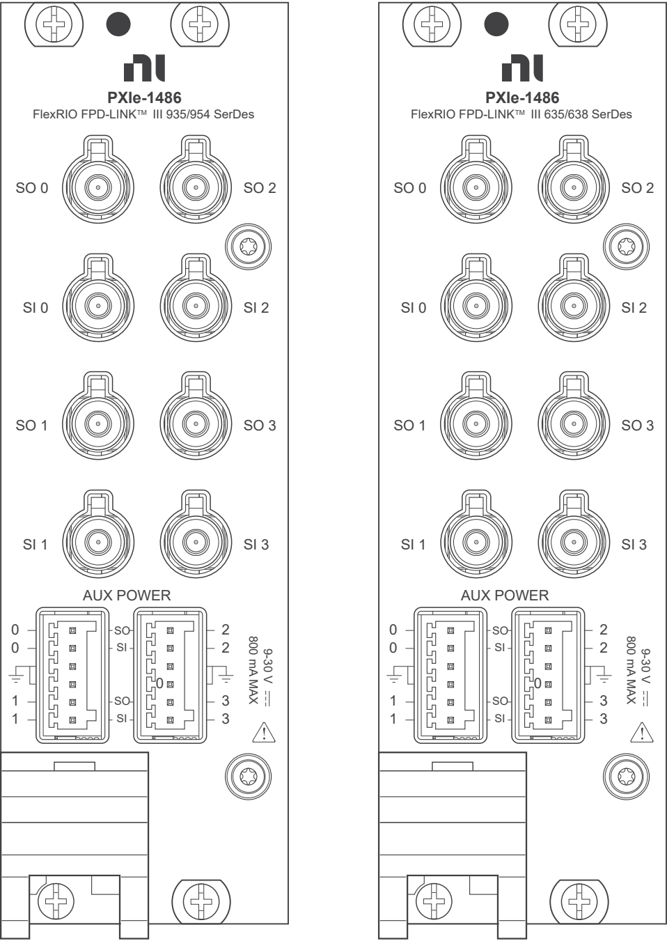
Figure 10. SerDes Front Panels
