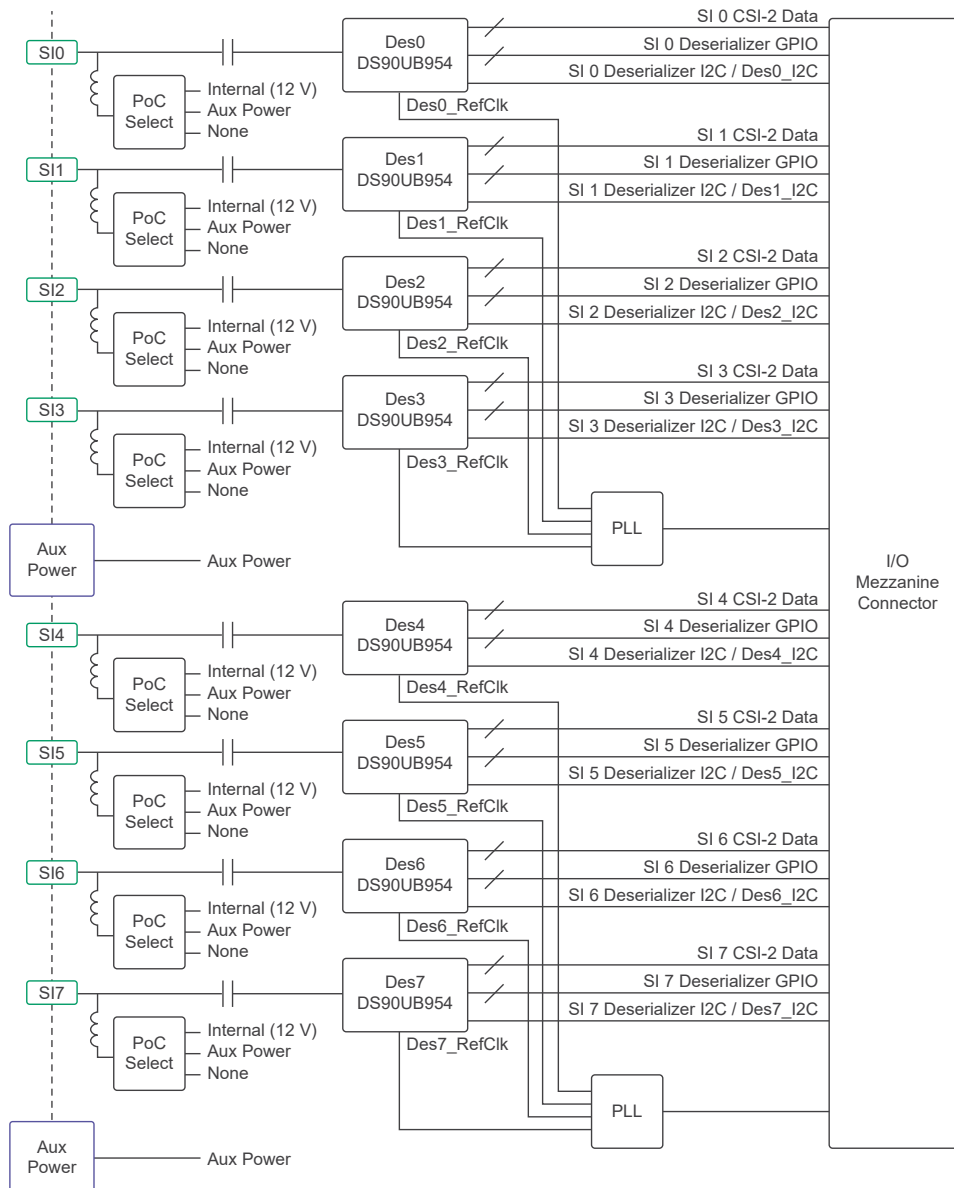
Figure 12. Deserializer Block Diagram
