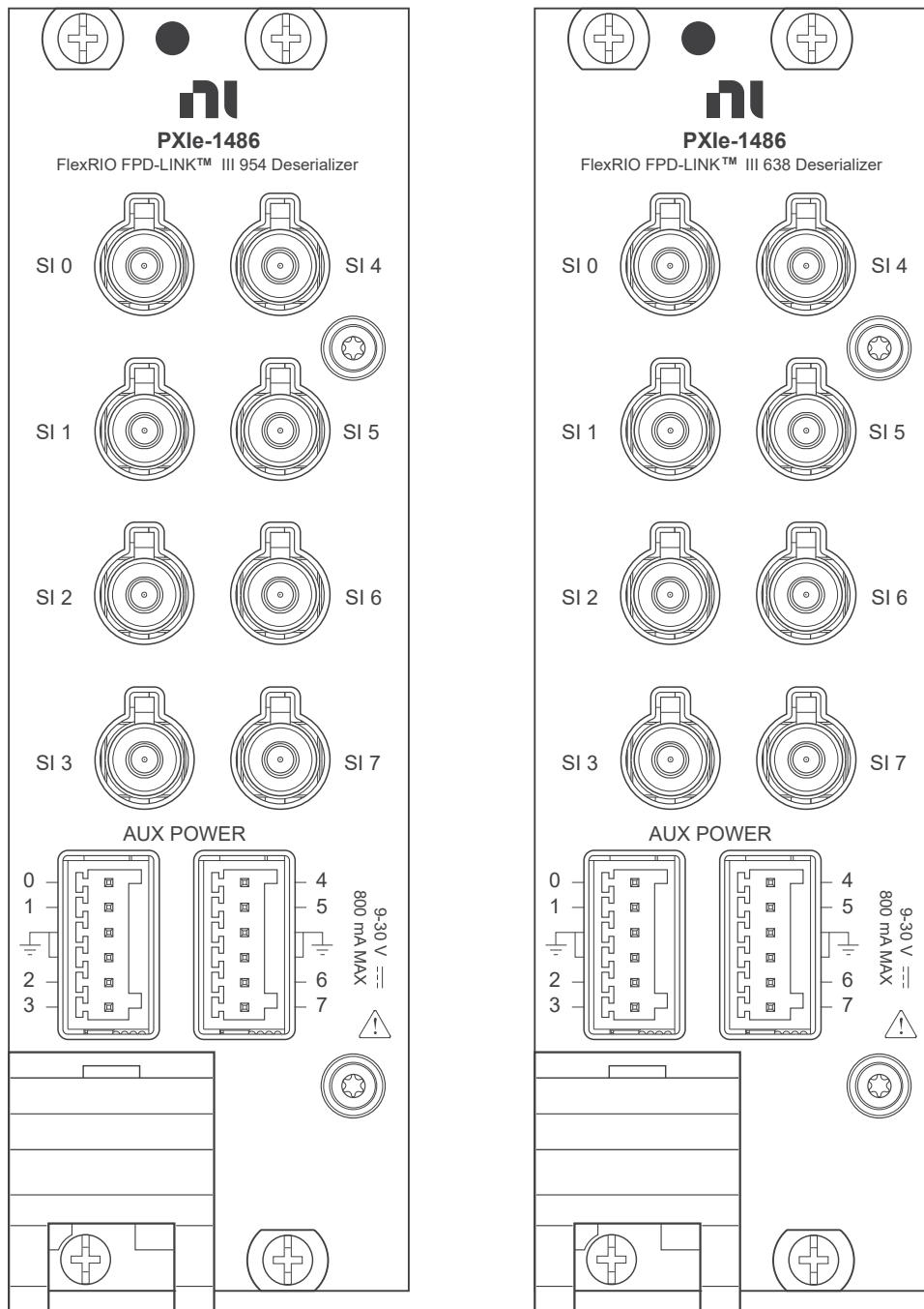
Figure 6. Deserializer Front Panels
