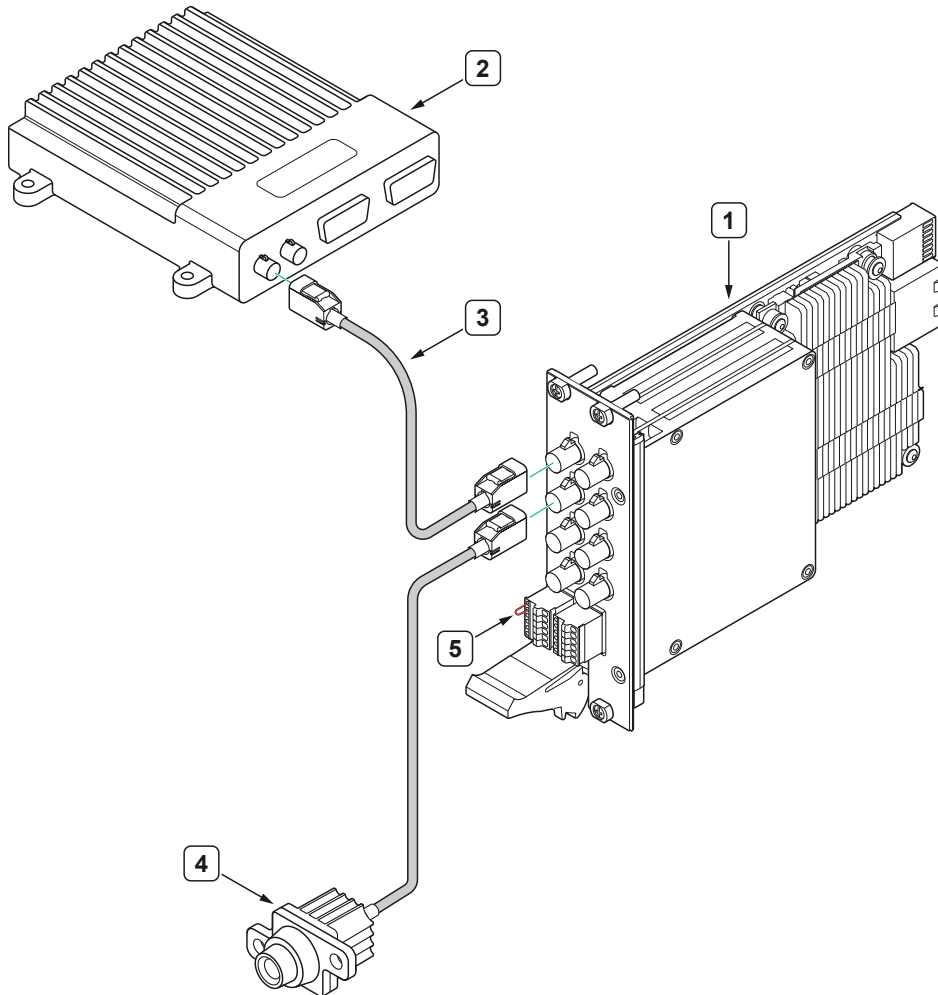
Figure 5. PXle-1486 SerDes
