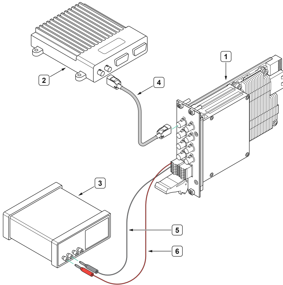
Figure 4. PXle-1486 Serializer
