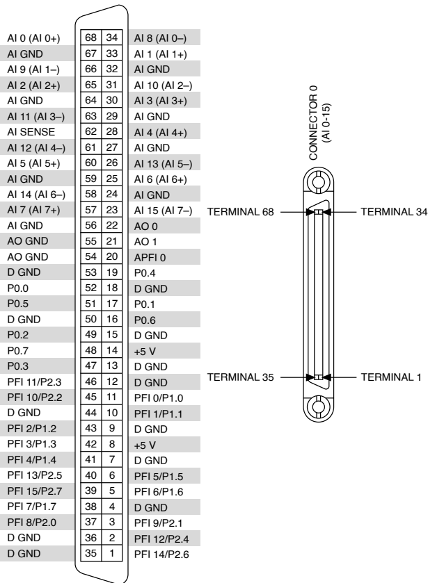
Figure 10. NI USB-6351 Pinout
