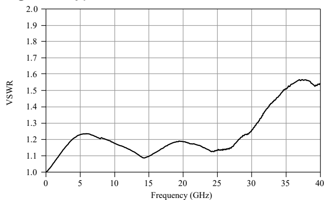
Figure 3. Typical VSWR
