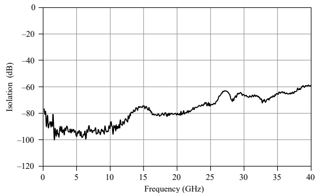
Figure 2. Typical Isolation
