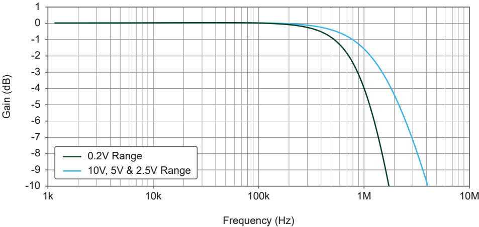
Figure 6. USB-6451 (Revision F and subsequent revisions) and USB-6451 (OEM) Small Signal Bandwidth versus Frequency
