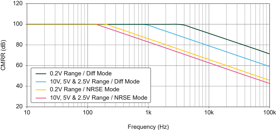
Figure 8. USB-6451 (Revision F and subsequent revisions) and USB-6451 (OEM) CMRR versus Frequency
