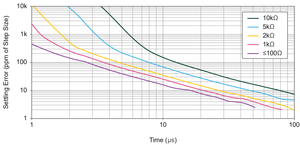
Figure 10. USB-6451 (Revision D) Settling Error versus Time for Different Source Impedances at the 0.2 V Input Range
