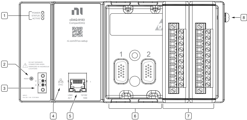
Figure 1. cDAQ-9183 Front Panel
