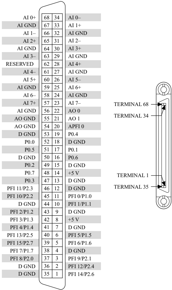
Figure 5. PCle-6346 Pinout
