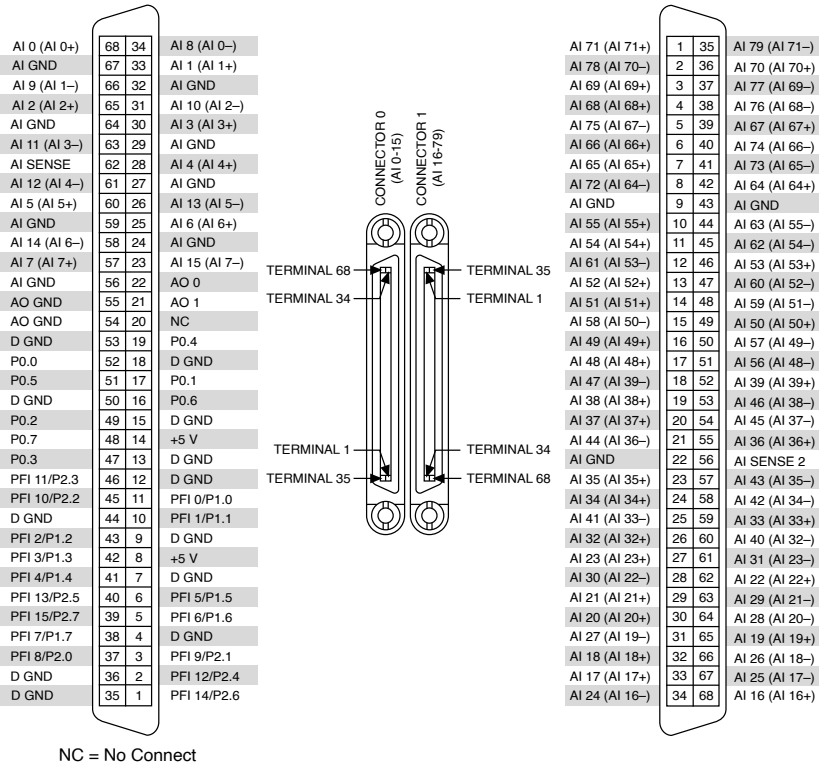
Figure 8. NI PCI/PXI-6225 Pinout
