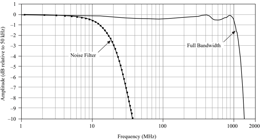
Figure 2. PCI-5154 Frequency Response, 5 V pk-pk through 0.1 V pk-pk Input Ranges, Measured
