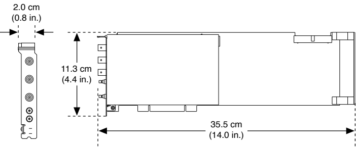
Figure 6. PCI-5154 Dimensions
