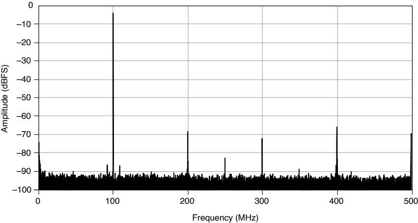
Figure 4. PCI-5154 Dynamic Performance, 2 V pk-pk Input Range, 100 MHz Input Signal, Measured
