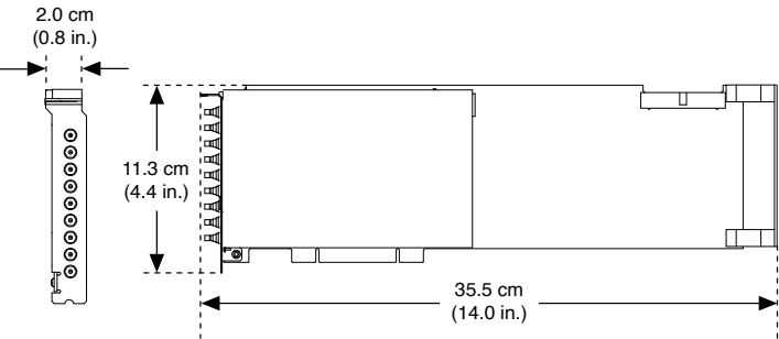
Figure 1. PCI-5105
