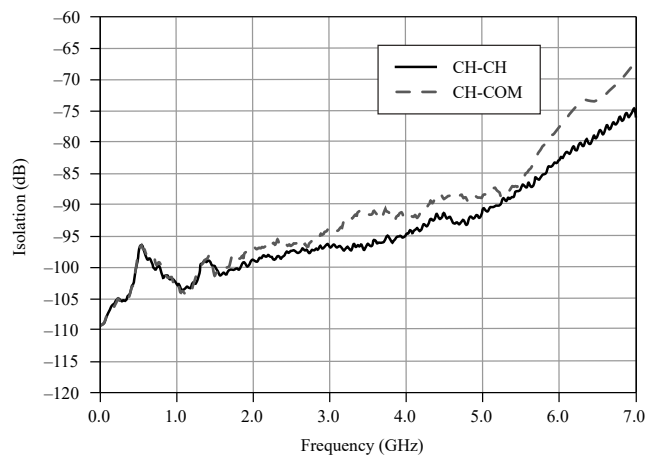
Figure 3. Typical Isolation
