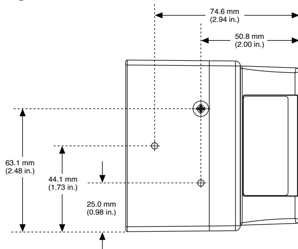
Figure 4. NI 9155 Side Dimensions
