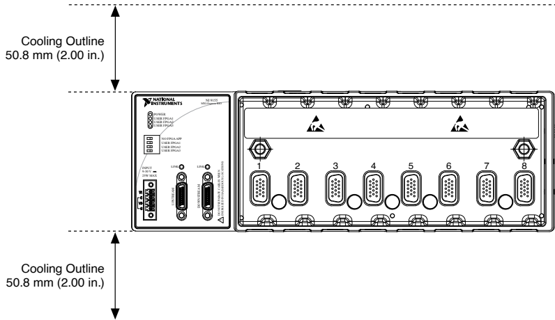
Figure 5. NI 9155 Cooling Dimensions
