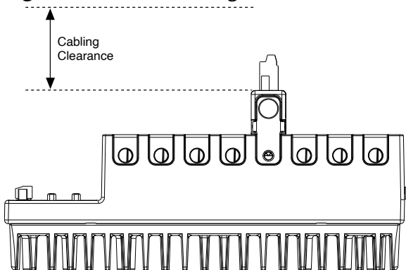
Figure 6. NI 9155 Cabling Clearance
