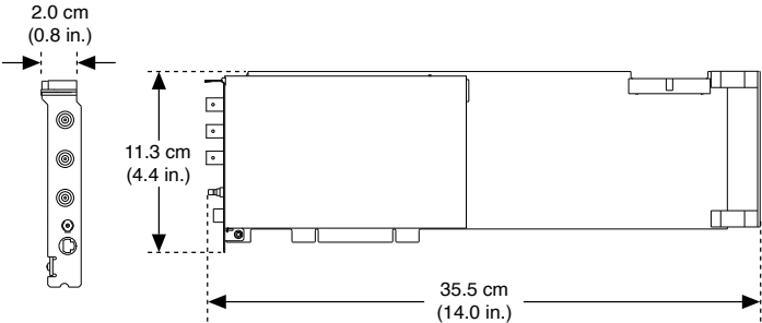
Figure 3. PCI-5114
