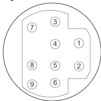
Figure 1. PCI-5114 9-Pin DIN Connector
