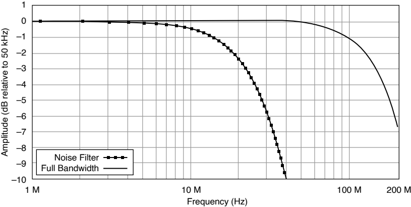
Figure 2. PCI-5114 Frequency Response, Measured
