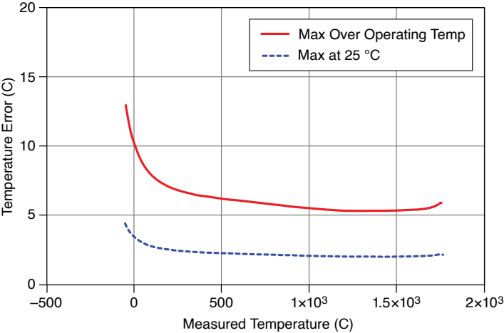
Figure 5. Temperature Error of Type N Thermocouple
