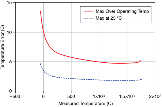
Figure 3. Temperature Error of Type R Thermocouple
