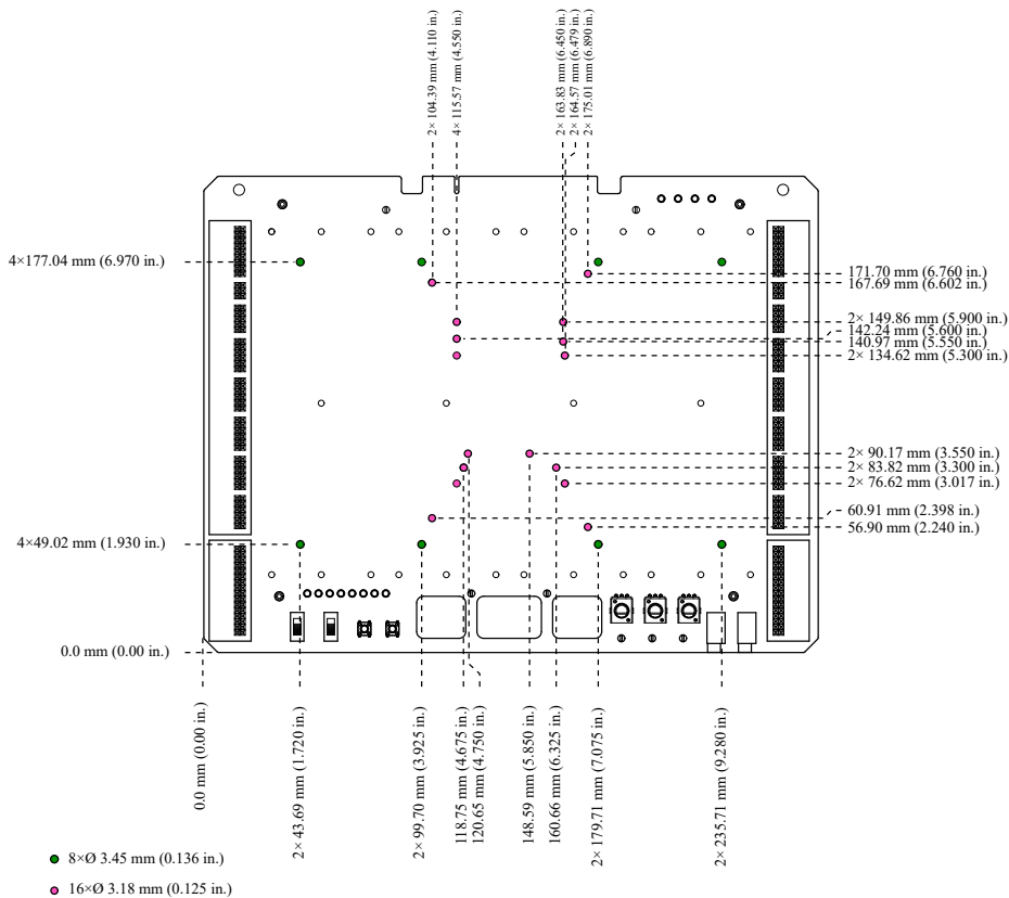
图 3. Prototyping Components Mounting Holes
