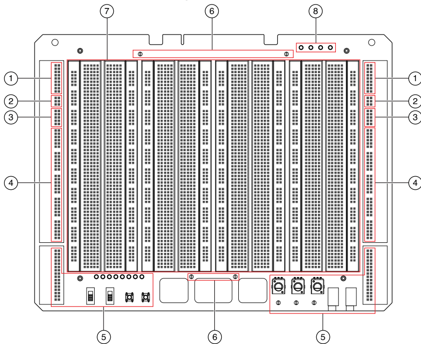
图 1. NI ELVIS III Prototyping Board
