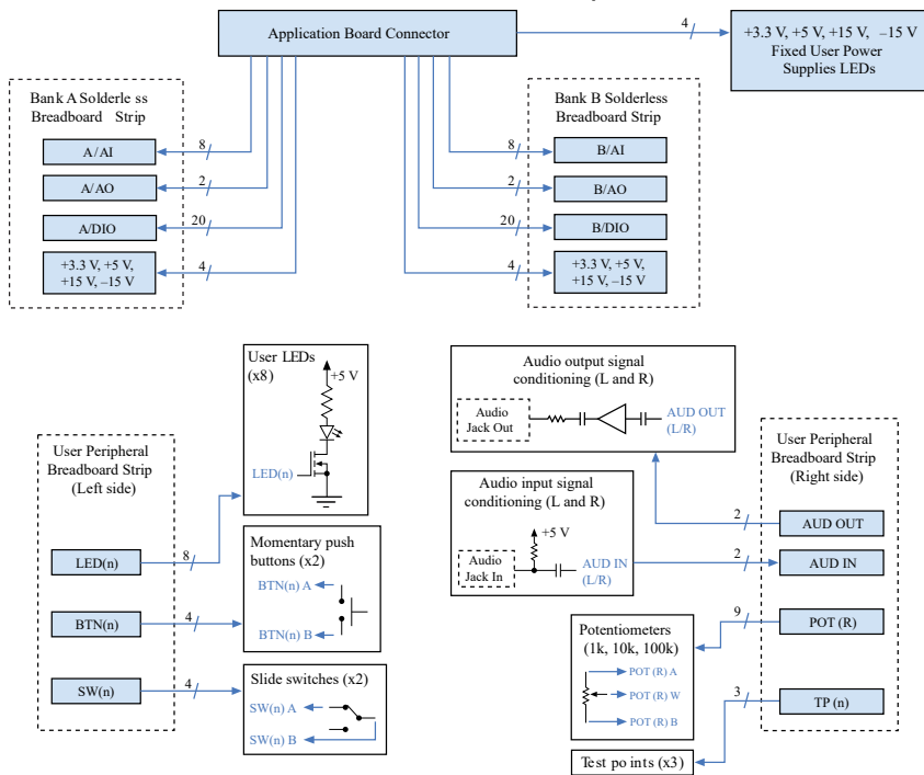
图 5. Hardware Architecture of User Peripherals
