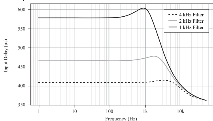
Figure 3. Butterworth Filter Input Delay (2nd Order, with 12.8 MHz Timebase, 500 Hz, 250 Hz, 125 Hz Filter)
