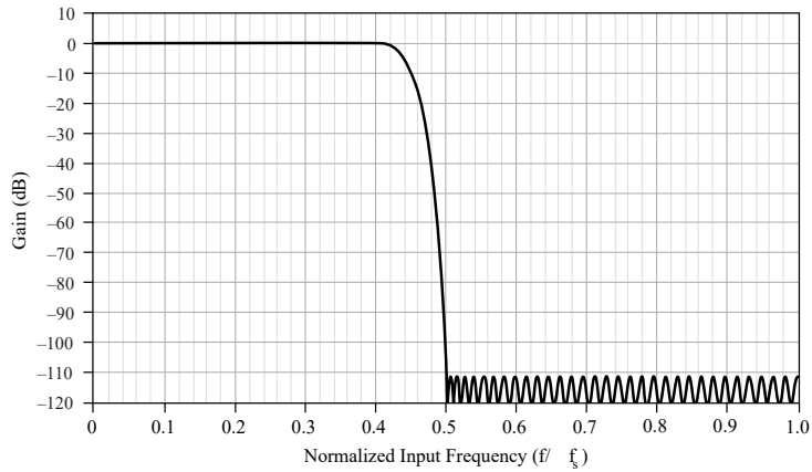
Figure 1. Brickwall Filter Magnitude Response
