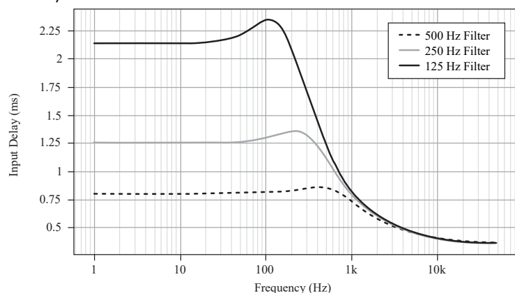
Figure 4. Butterworth Filter Input Delay (4th Order, with 12.8 MHz Timebase, 4 kHz, 2 kHz, 1 kHz Filter)
