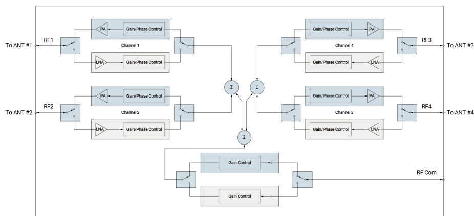
Figure 2. 5G Beamformer RF Diagram (4 channels)
