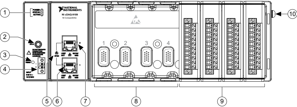
Figure 2. cDAQ-9189 Front Panel
