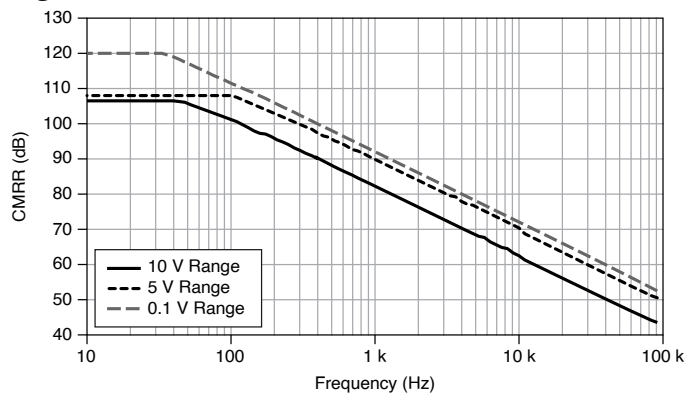
Figure 3. AI CMRR
