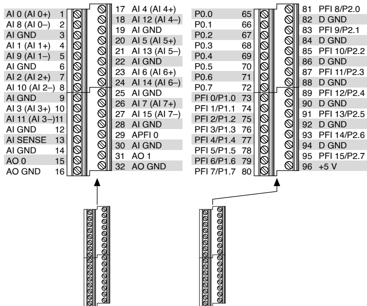
Figure 10. NI USB-6251 Screw Terminal Pinout
