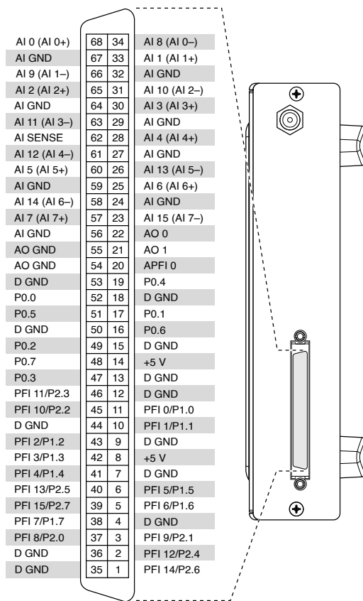
Figure 12. NI USB-6251 Mass Termination Pinout
