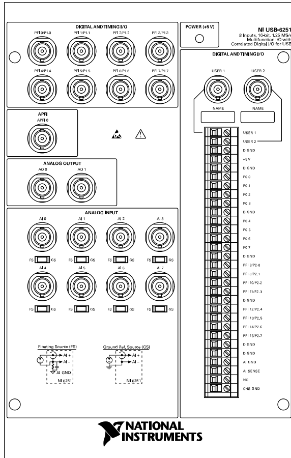
Figure 11. NI USB-6251 BNC Front Panel and Pinout
