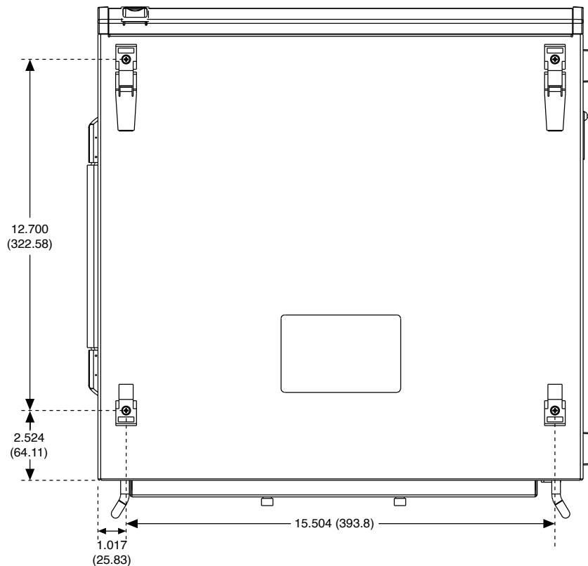
Figure 1. PXle-1075 Chassis Dimensions (Bottom)
