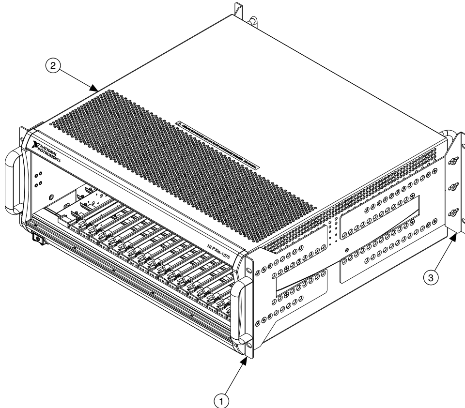
Figure 3. NI Chassis Rack Mount Kit Components
