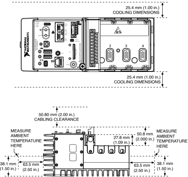
Figure 1. NI cDAQ-9136 Temperature, Cooling, and Cabling Dimensions
